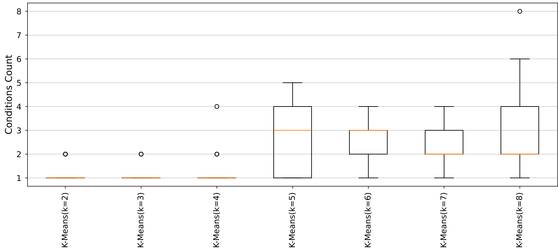
YARA Rules Conditions Count Distribution (Cluster16_Size8 dataset)
